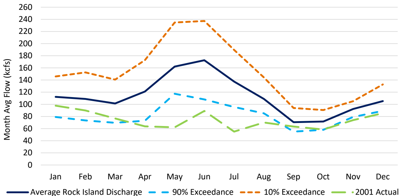
Figure 21 Monthly average Wanapum inflow, 1996-2025, kcfs
