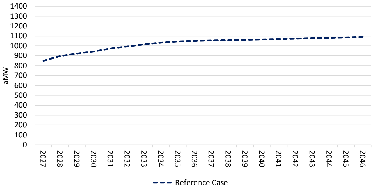
Figure 7 Grant PUD reference case load forecast, 2027-2046, aMW
