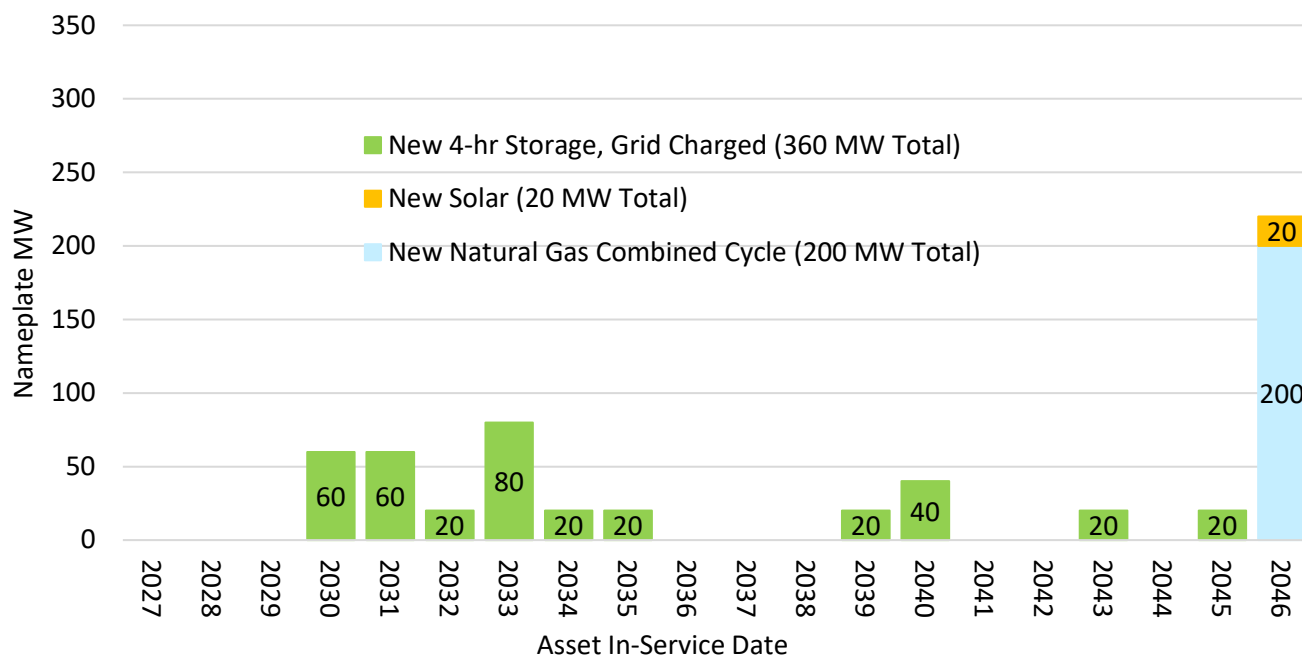
Figure 52 Carbon policy sensitivity case acquisition plan from ARS modeling, 2027-2046
