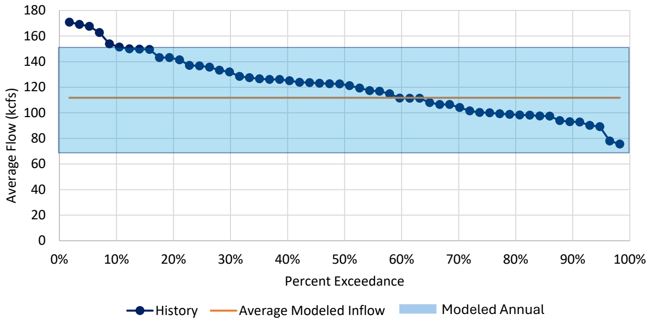
Figure 19 Northwest River Forecast Center water year runoff volumes, measured below Priest Rapids Dam, 1971–2026, and modeled annual average flow, kcfs
