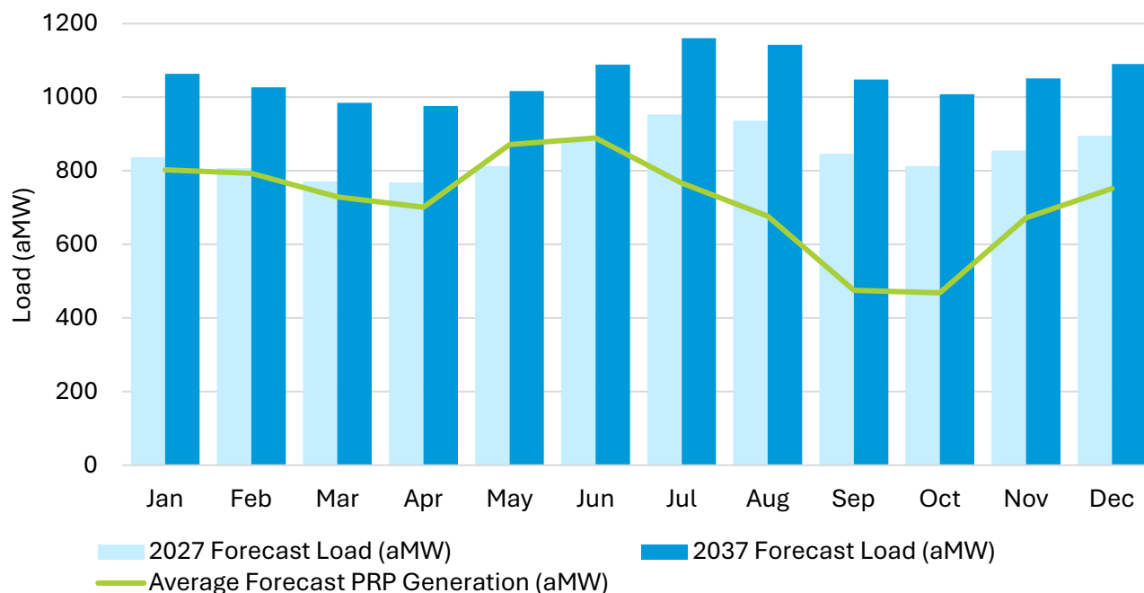
Figure 23 Forecast monthly load, 2027 and 2037, aMW vs. forecast average monthly Priest Rapids Project generation, 2027-2046, aMW
