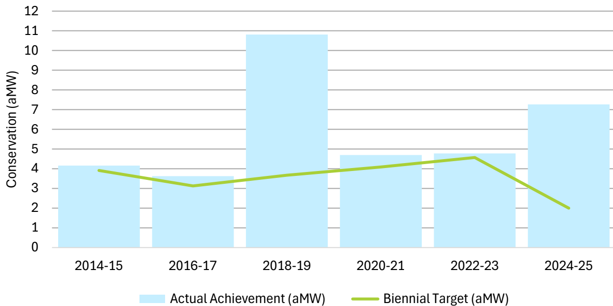
Figure 53 Grant PUD historic conservation targets and achievements, 2014-2025, aMW
