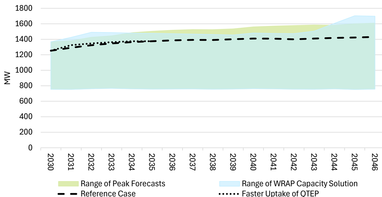
Figure 4 Recommended portfolio meets WRAP requirements across a broad range of load futures, 2025-2046, MW
