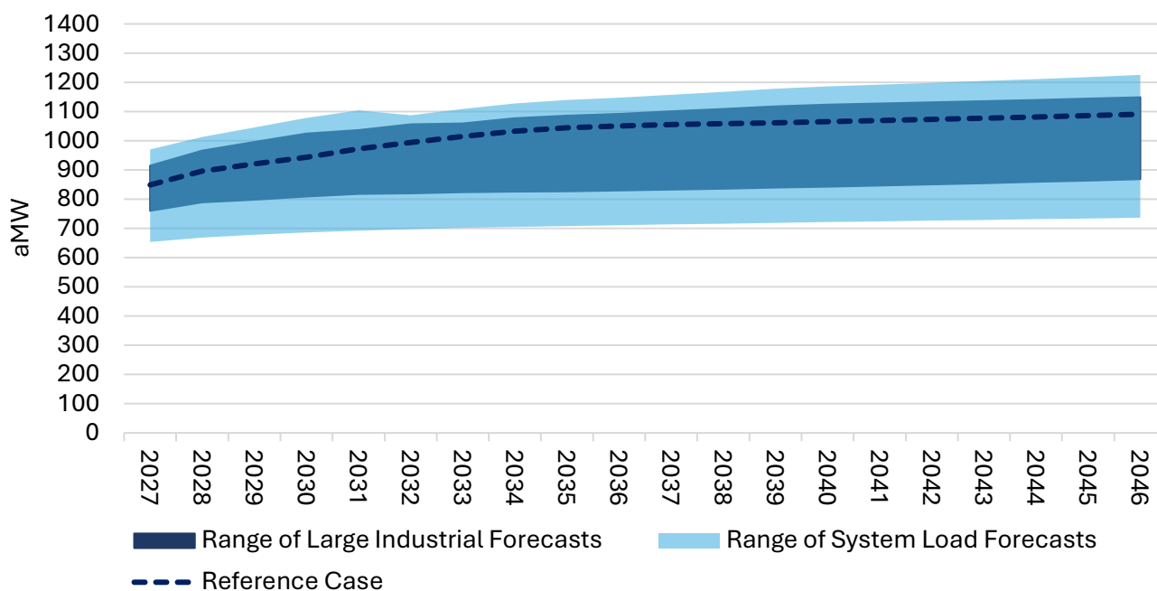
Figure 15 Range of Grant PUD load forecasts with overlay of range of Large Industrial customer load forecasts, 2027-2046, aMW
