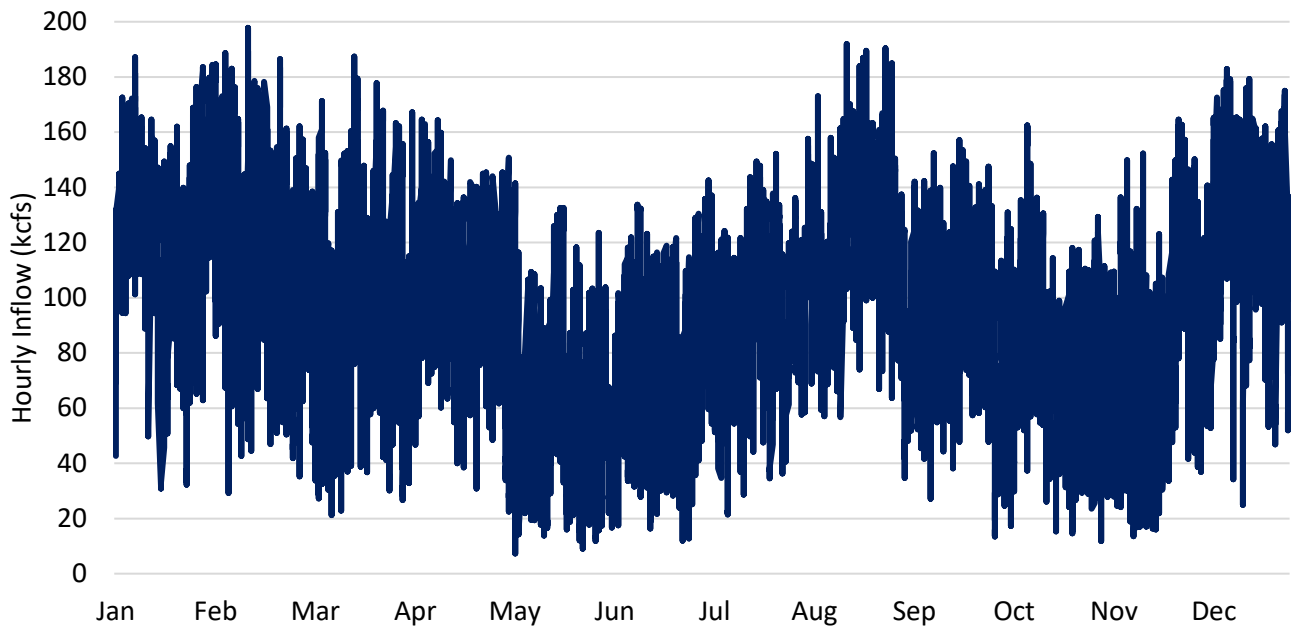
Figure 25 Hourly Wanapum inflows, 2025, kcfs
