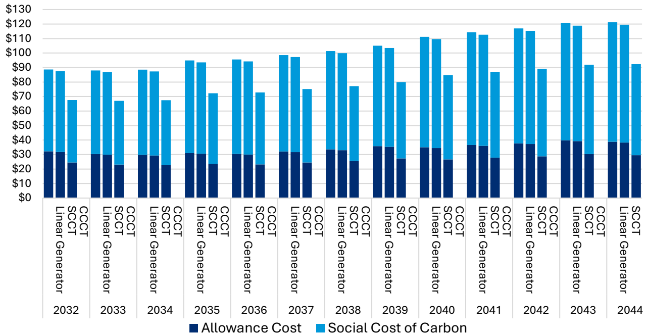
Figure 27 Carbon policy compliance cost forecast for natural gas-fired generators, at generator full load, 2032-2044, $/MWh
