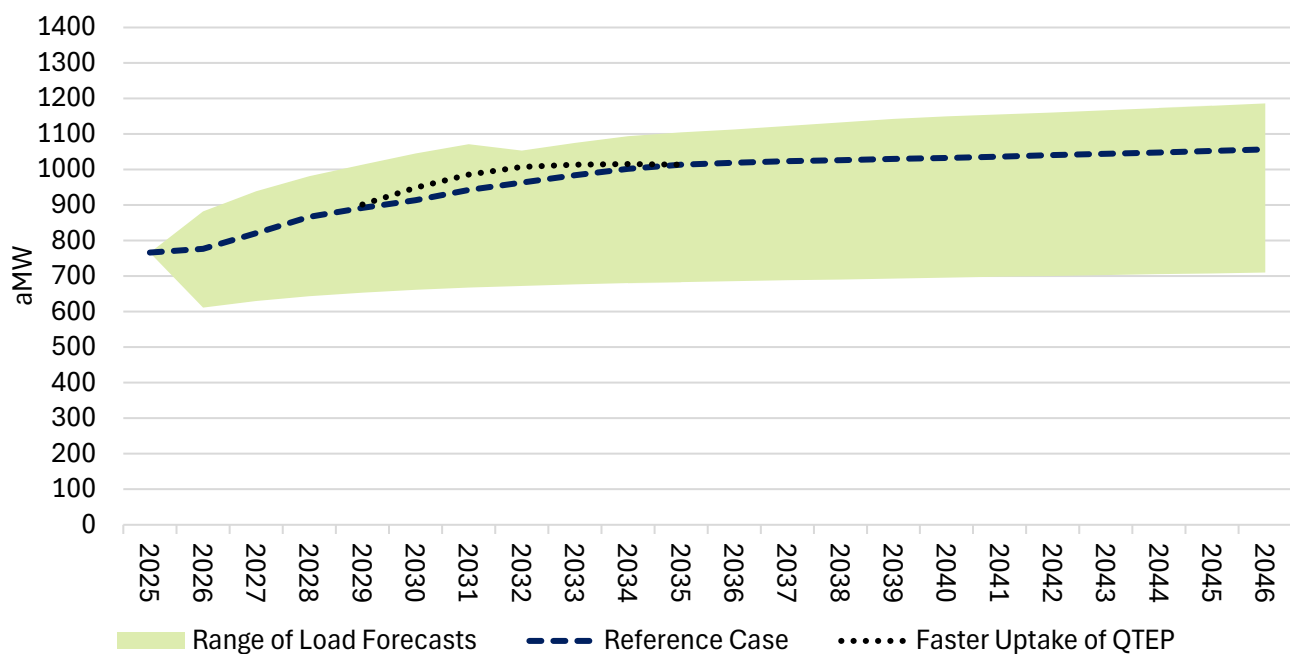
Figure 2 Range of load forecasts considered in 2026 IRP analysis, 2027-2046, aMW
