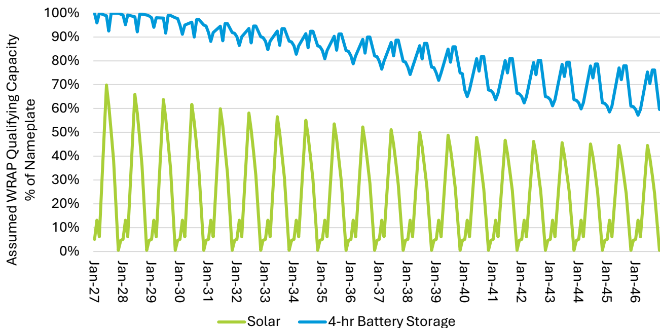
Figure 47 Assumed WRAP qualifying capacity contribution, solar and 4-hour storage, 2027-2046
