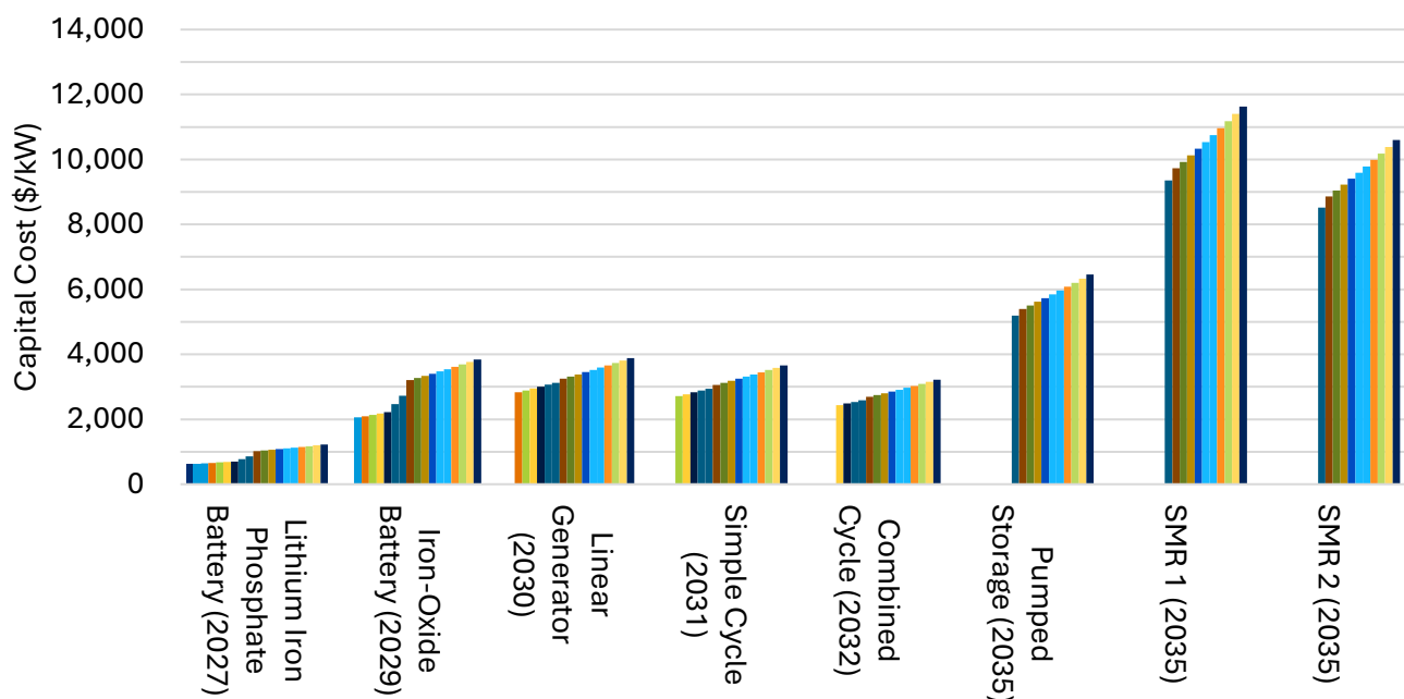
Figure 17 Forecast capital costs by technology type for candidate resources evaluated as ownership options, 2027-2046, nominal dollars
