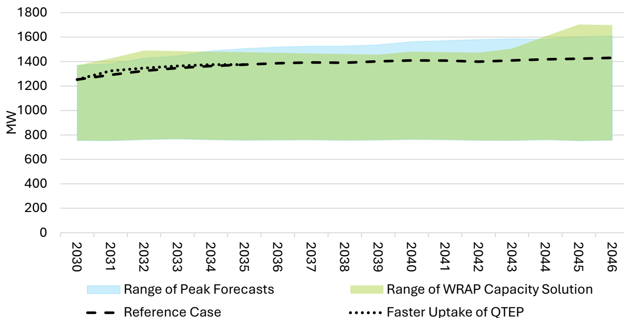
Figure 48 Recommended portfolio meets WRAP requirements across a wide range of load futures, 2025-2046, MW
