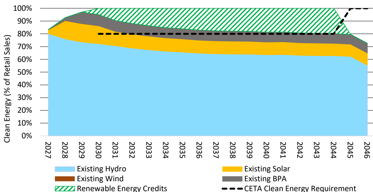
Figure 29 Annual CETA compliant clean energy available from existing portfolio, percent of retail sales, 2027-2046
