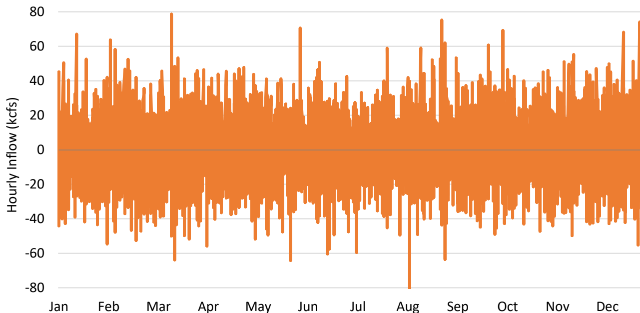
Figure 26 Hour-to-hour changes in Wanapum inflows, 2025, kcfs
