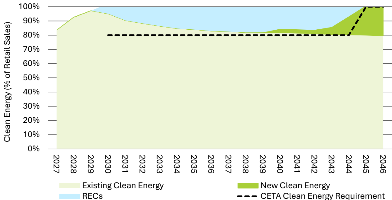
Figure 50 Recommended plan meets CETA requirements through use of existing portfolio, new clean energy resources, and RECs, 2027-2046
