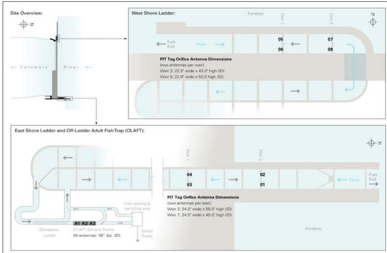
Figure 3 Plan view of upper regions of the fishway at Priest Rapids Dam showing location of PIT-tag detection antennas and associated identification number.
