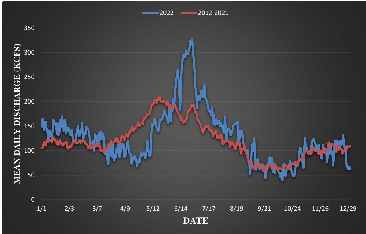
Figure 4 Comparison of 2022 vs. previous 10-year average of mean daily discharge values measured at the U.S. Geological Survey (USGS) streamflow gage #12472800 located 2.6 river miles below Priest Rapids Dam, Priest Rapids Hydroelectric Project, mid-Columbia River, WA.
