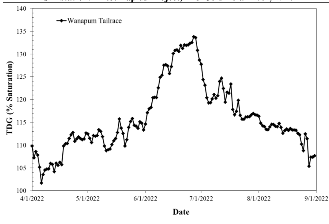
Figure 7 Total dissolved gas values (average of the 12-highest hourly TDG values in a day) from the 2022 fish-spill season recorded at the Wanapum Dam tailrace FSM station. Priest Rapids Project, mid-Columbia River, WA.
