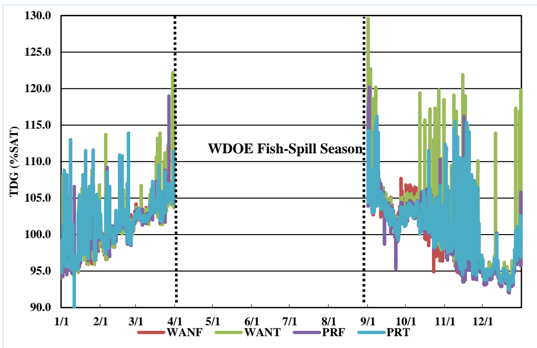
Figure 5 Hourly total dissolved gas values from the 2022 non-fish spill season, Priest Rapids Hydroelectric Project, mid-Columbia River, WA.
