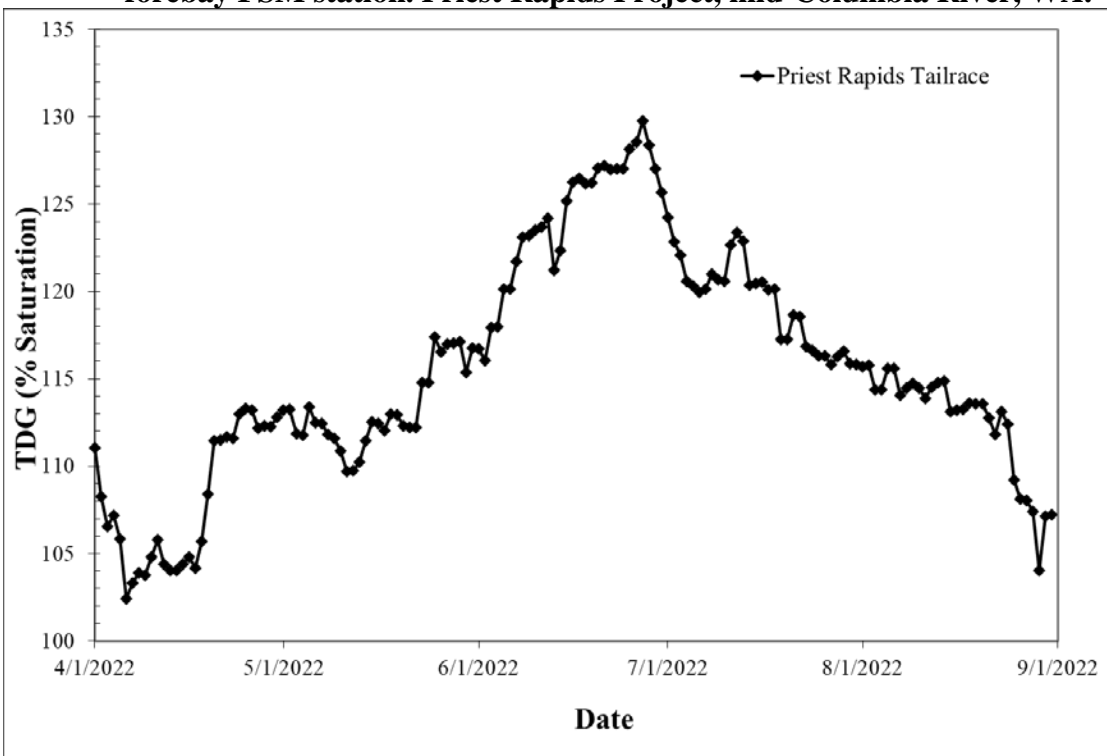
Figure 9 Total dissolved gas values (average of the 12-highest hourly TDG values in a day) from the 2022 fish-spill season recorded at the Priest Rapids Dam tailrace FSM station. Priest Rapids Project, mid-Columbia River, WA.
