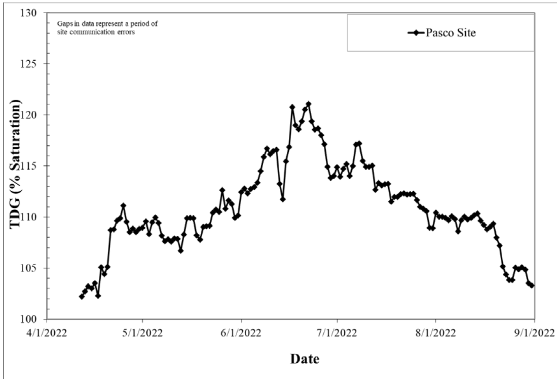
Figure 10 Total dissolved gas values (average of the 12-highest hourly TDG values in a day) from the 2022 fish-spill season recorded at the Pasco FSM station, mid-Columbia River, WA.
