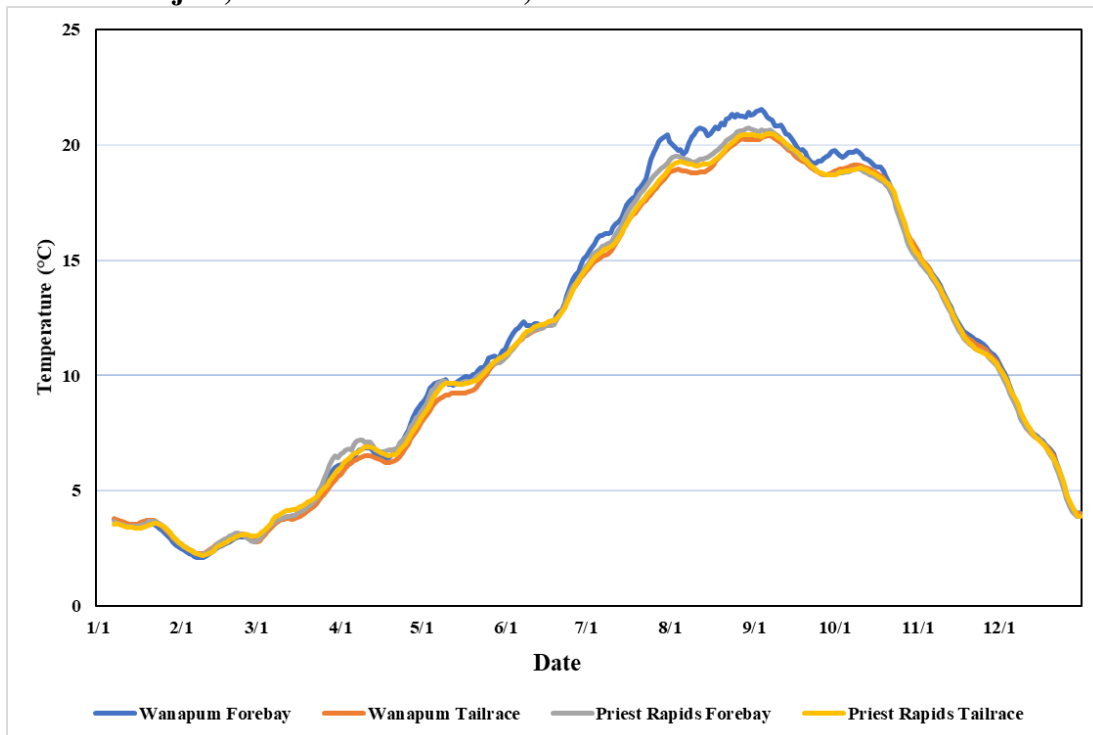
Figure 12 Seven-day rolling average of daily maximum temperatures (7-DADMax) recorded at each fixed-site monitoring station (FSM station) in 2022, Priest Rapids Hydroelectric Project, mid-Columbia River, WA.
