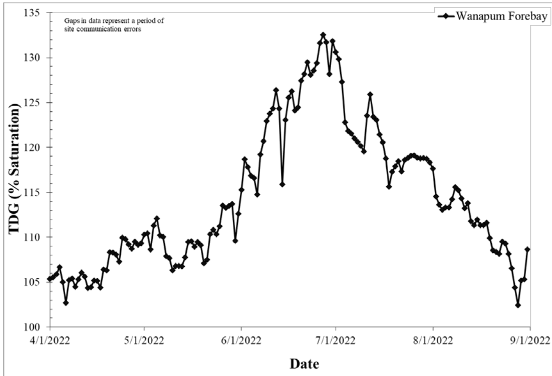
Figure 6 Total dissolved gas values (average of the 12-highest hourly TDG values in a day) from the 2022 fish-spill season recorded at the Wanapum Dam forebay FSM station. Priest Rapids Project, mid-Columbia River, WA.
