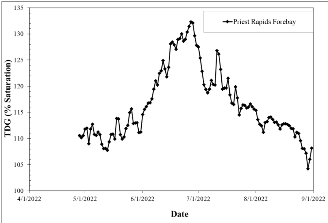
Figure 8 Total dissolved gas values (average of the 12-highest hourly TDG values in a day) from the 2022 fish-spill season recorded at the Priest Rapids Dam forebay FSM station. Priest Rapids Project, mid-Columbia River, WA.
