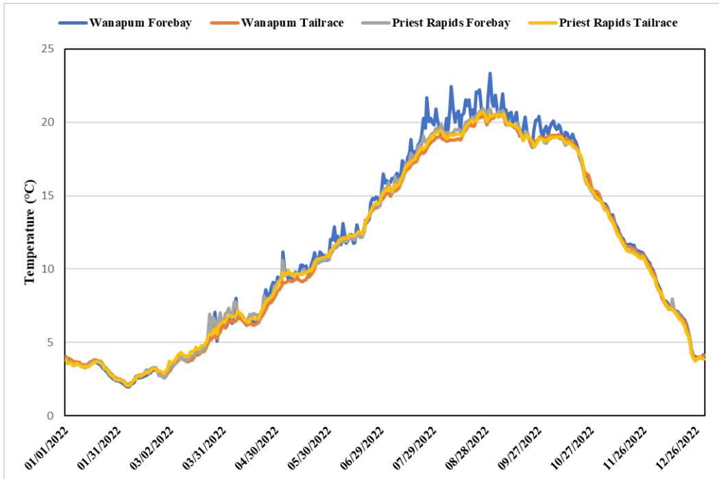
Figure 11 Daily maximum (1-DMax) water temperature values recorded at each fixed-site monitoring station (FSM station) in 2022, Priest Rapids Hydroelectric Project, mid-Columbia River, WA.
